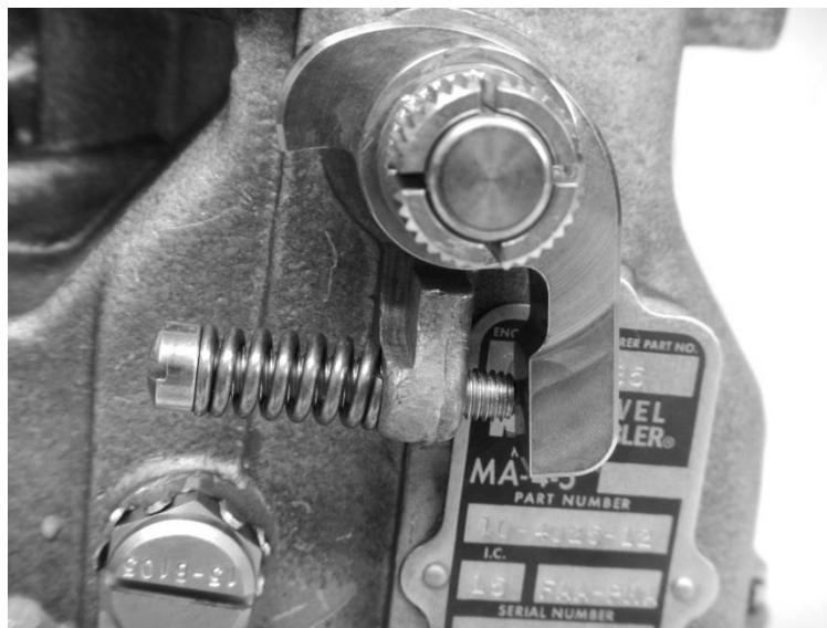
Figure 5-10a: Idle Position
