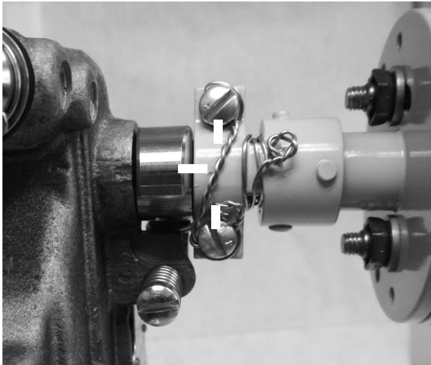
Figure 5-10f: Application of Anti-Sabotage Lacquer
