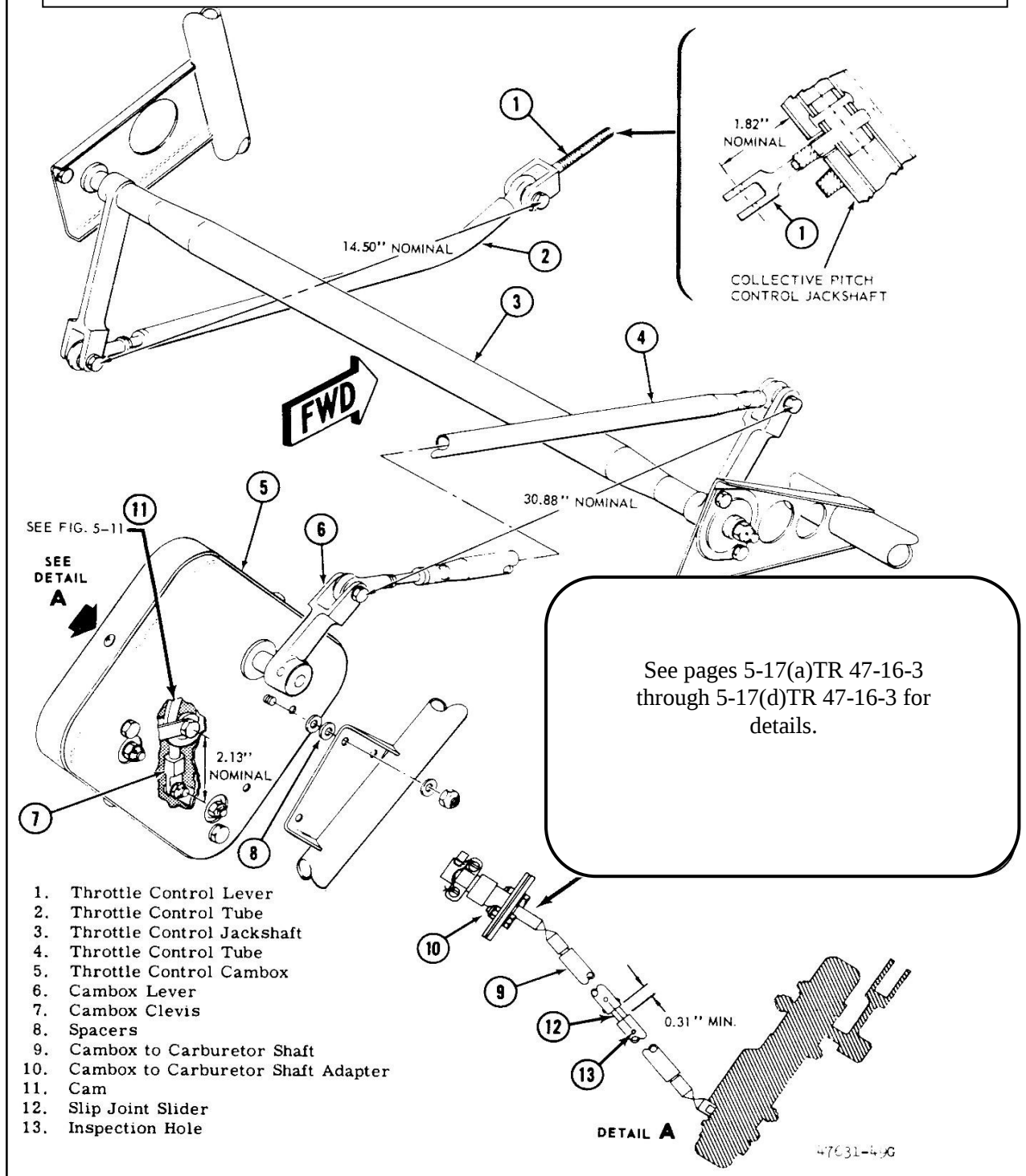
Figure 5-10. Throttle Control Installation
